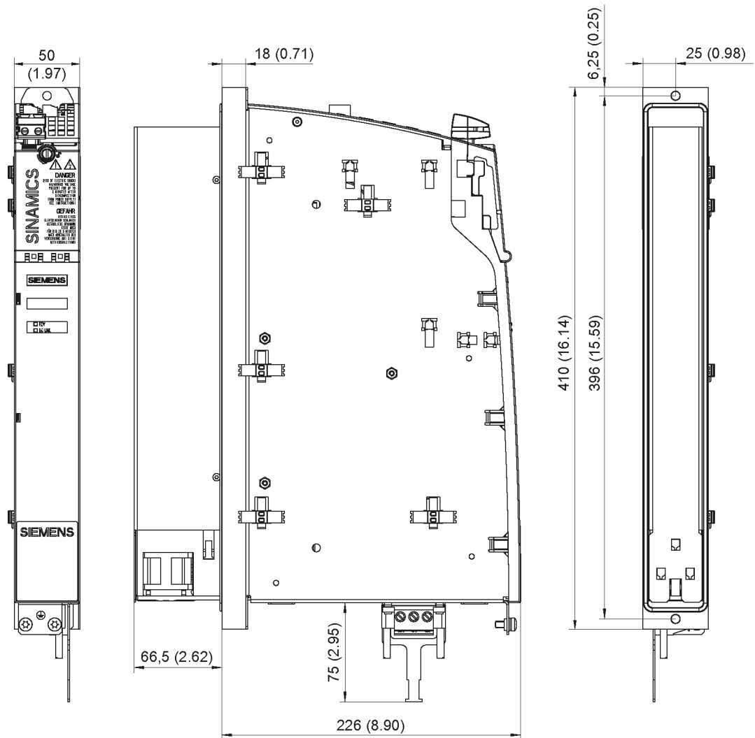
Figure 4-79 Dimension drawing of 5 kW and 10 kW Smart Line Modules with external air cooling, all dimensions in mm and (inches)
